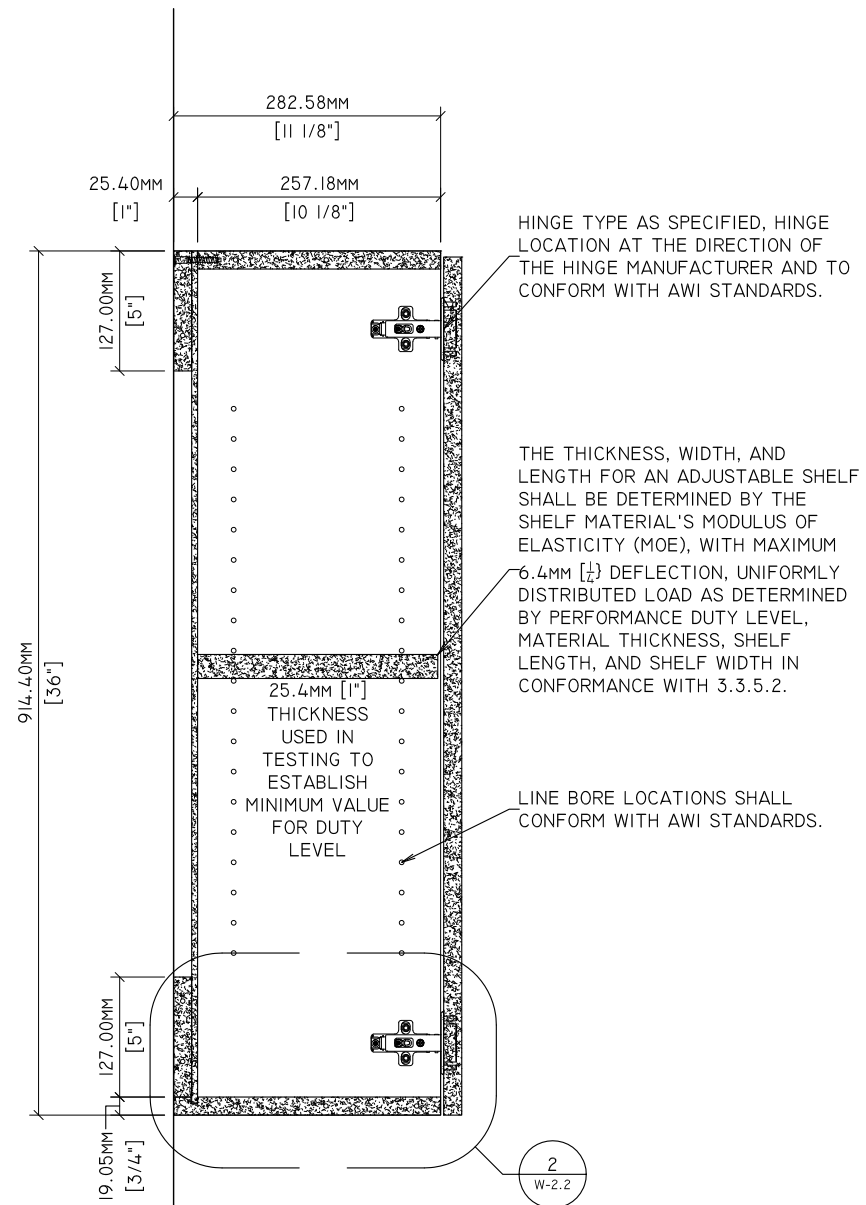
1 SECTION W-2.2 1-1/2" = 1'-0"
