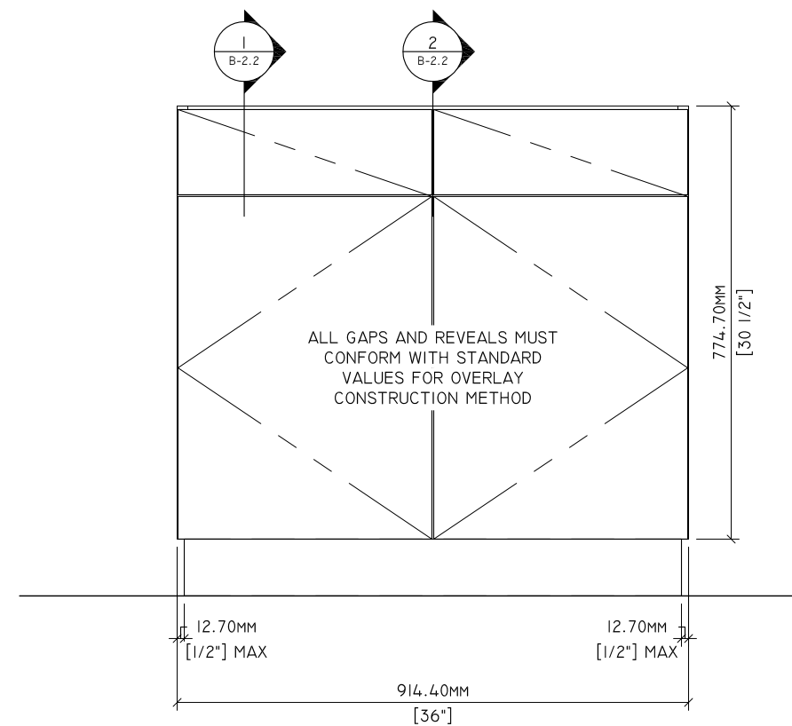
3 B-2.1 ELEVATION 1" = 1'-0"
