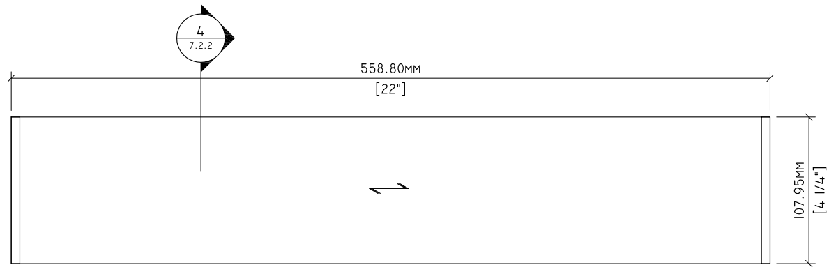
1 ELEVATION 7.2.2 3" = 1'-0"
