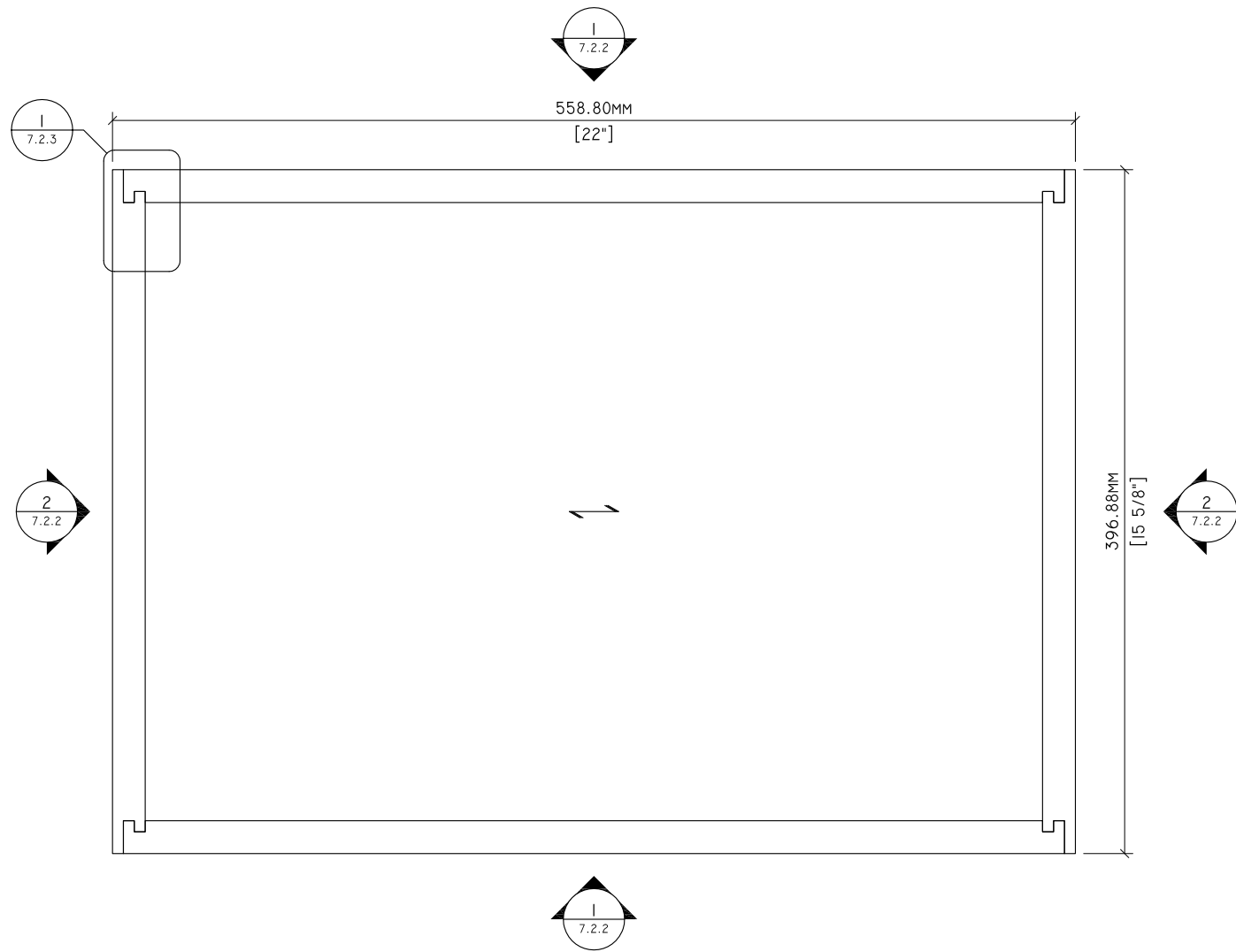
1 7.2.1 PLAN 3" = 1'-0"
