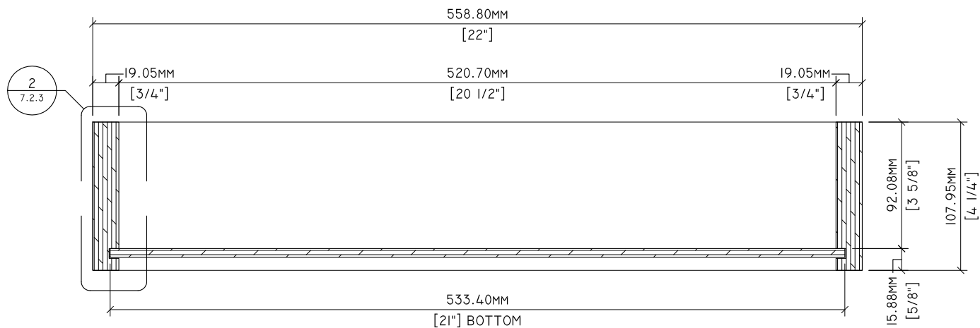
3 SECTION 7.2.2 3" = 1'-0"
